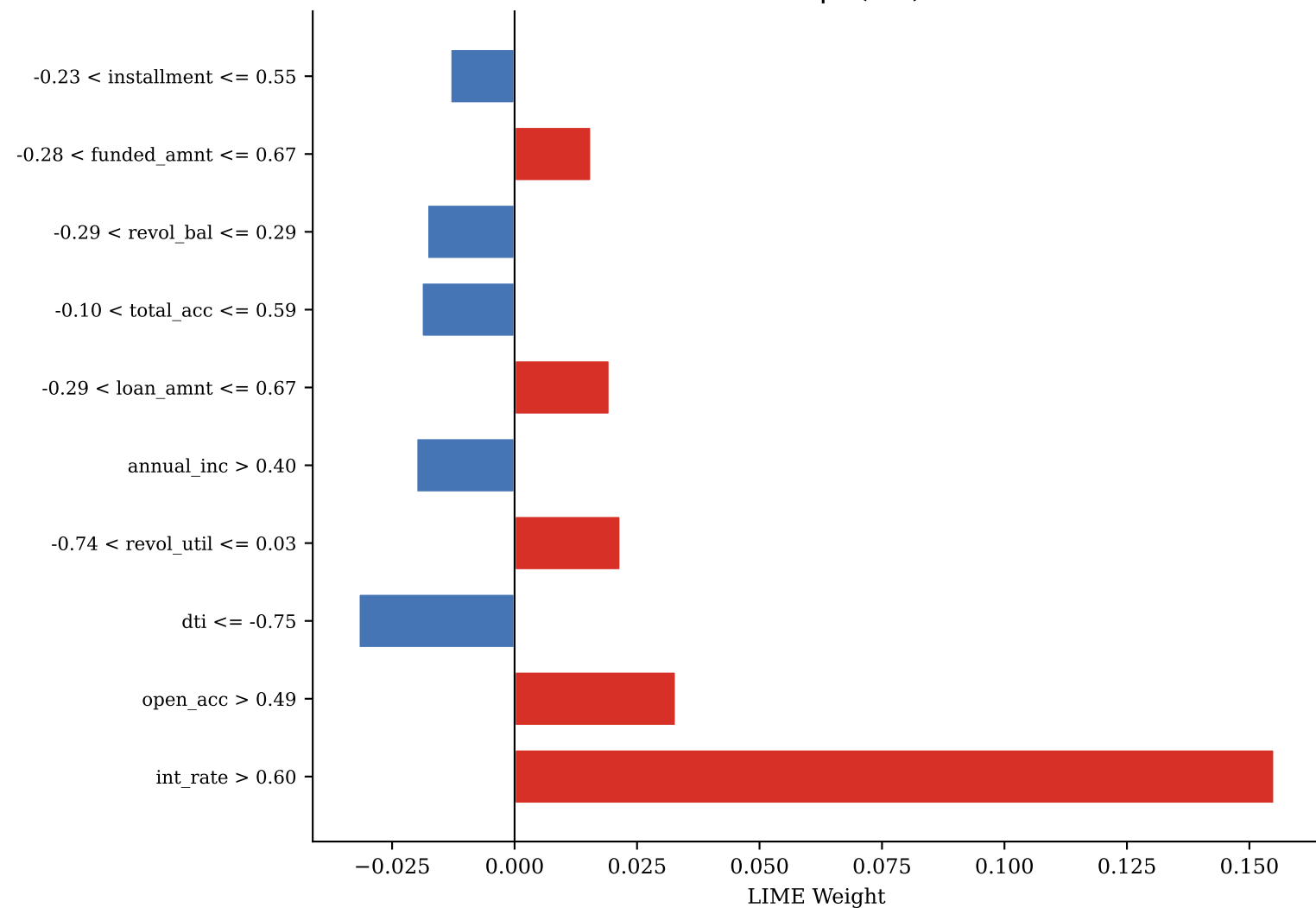
TN — idx 1677 | P(def)=0.140
