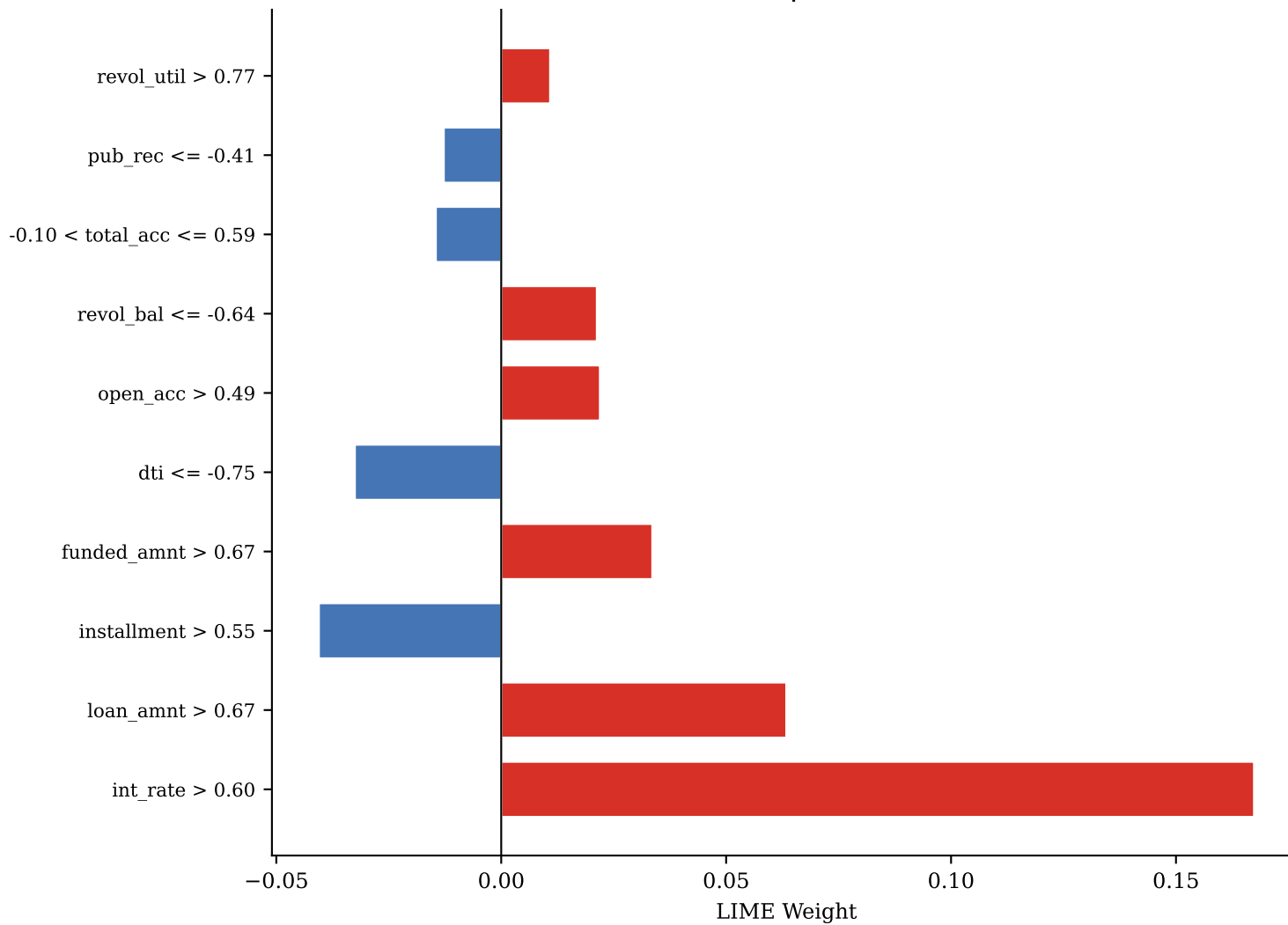
FN — idx 2309 | P(def)=0.140
