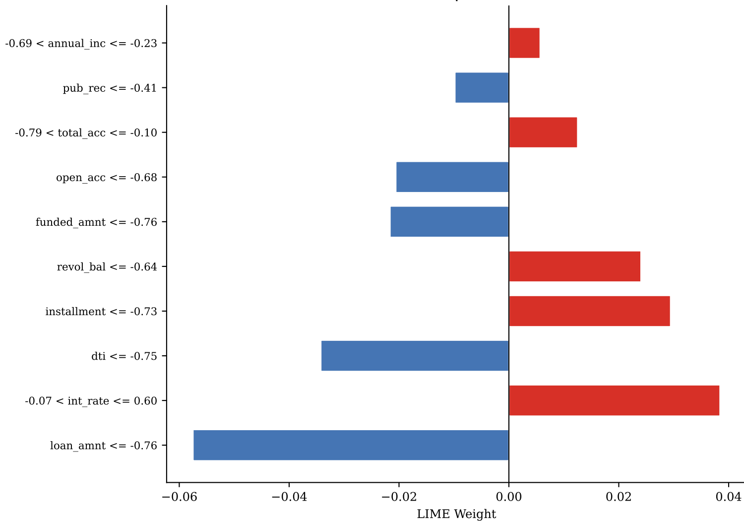
TN — idx 140 | P(def)=0.140
