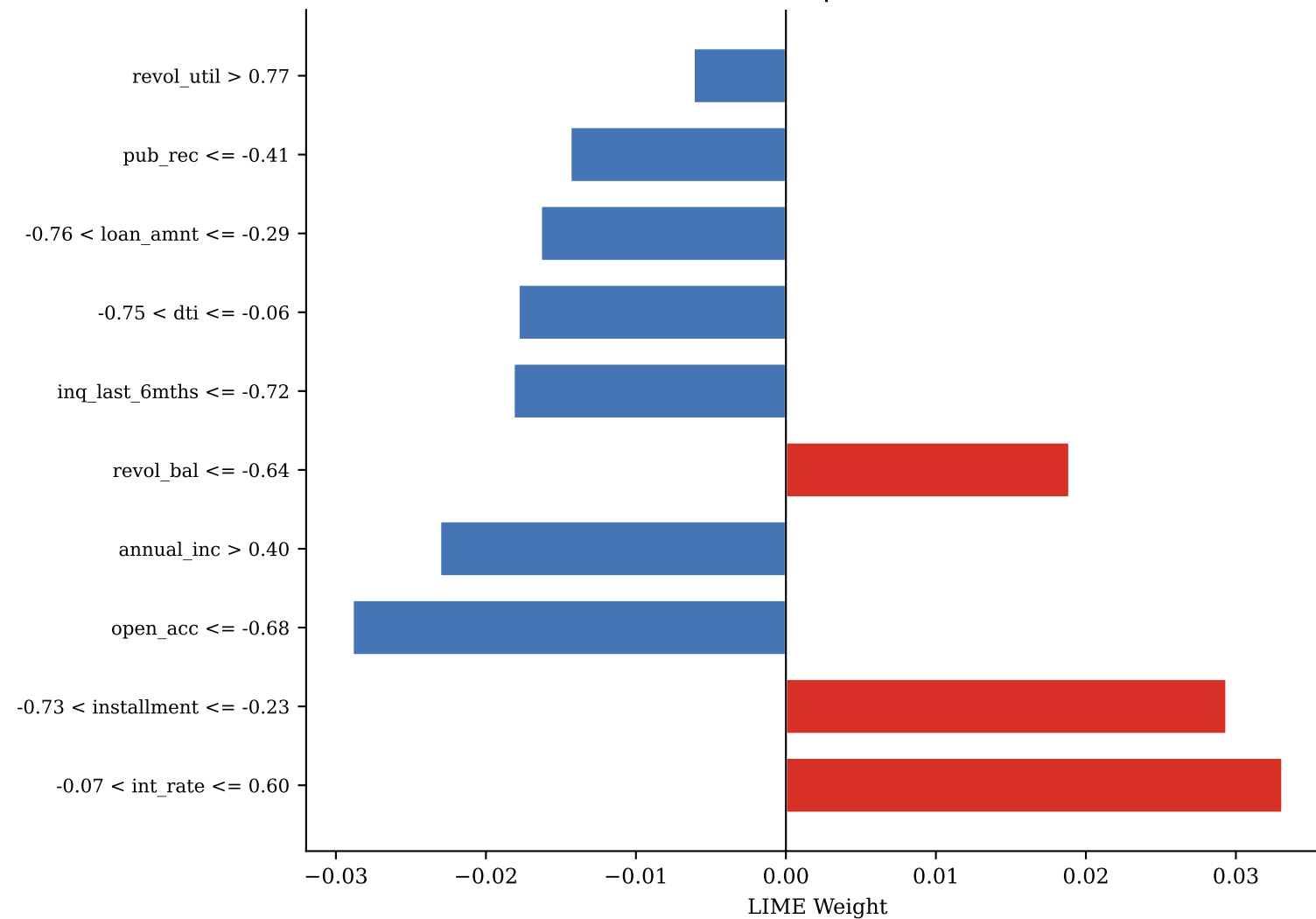
FN — idx 2309 | P(def)=0.140
