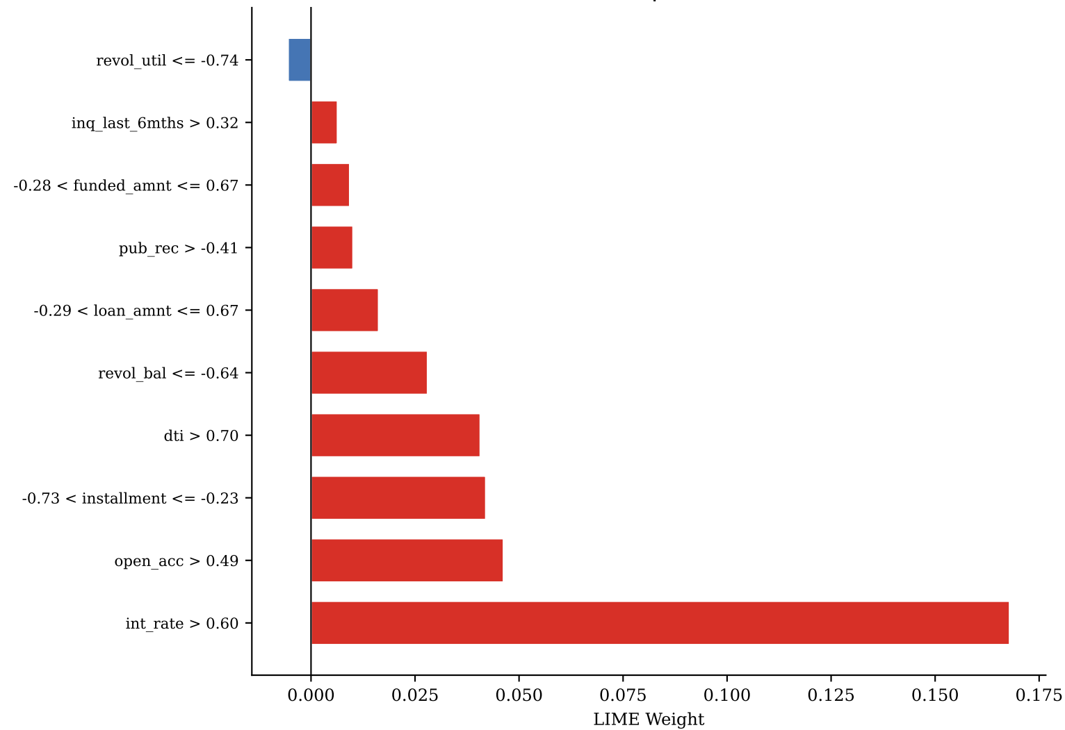
FN — idx 6234 | P(def)=0.150
