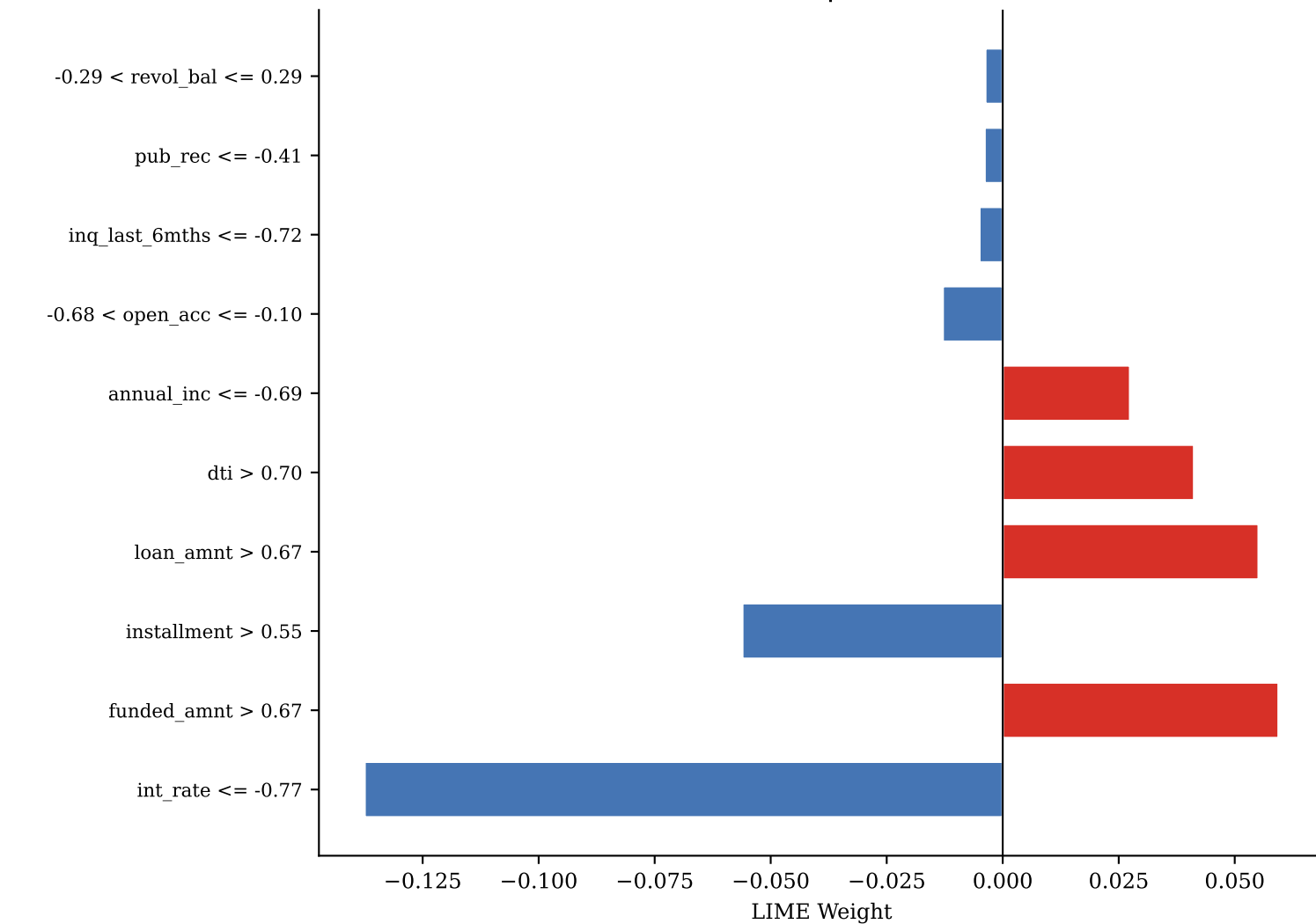
FN — idx 6234 | P(def)=0.150
