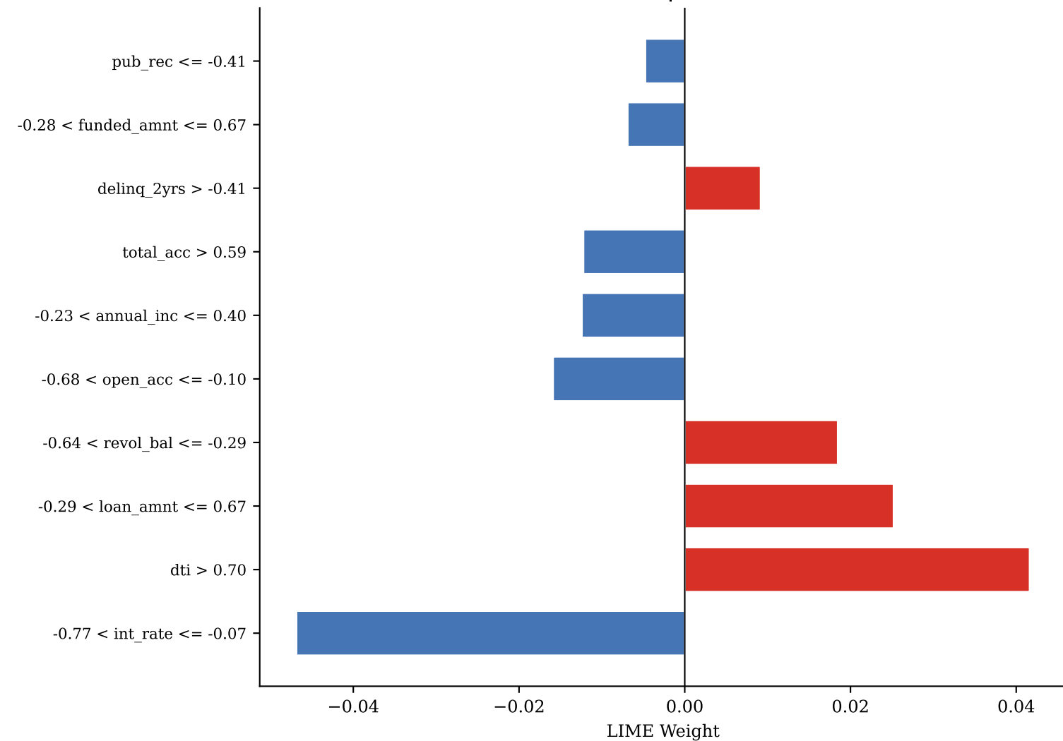
TN — idx 4562 | P(def)=0.150
