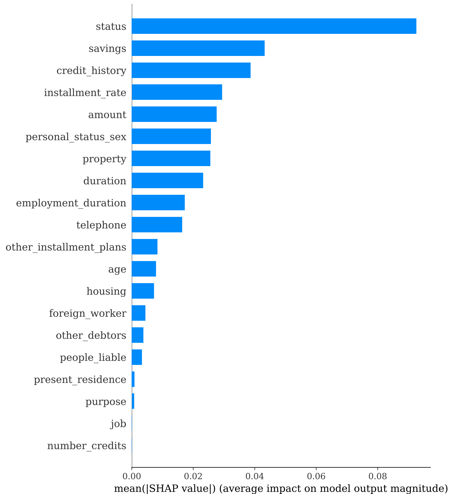
Mean |SHAP| — Logistic Reg.
