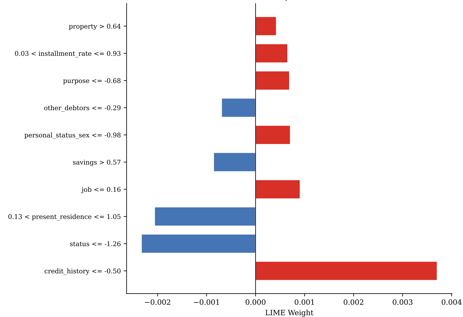
FN — idx 50 | P(def)=0.497
