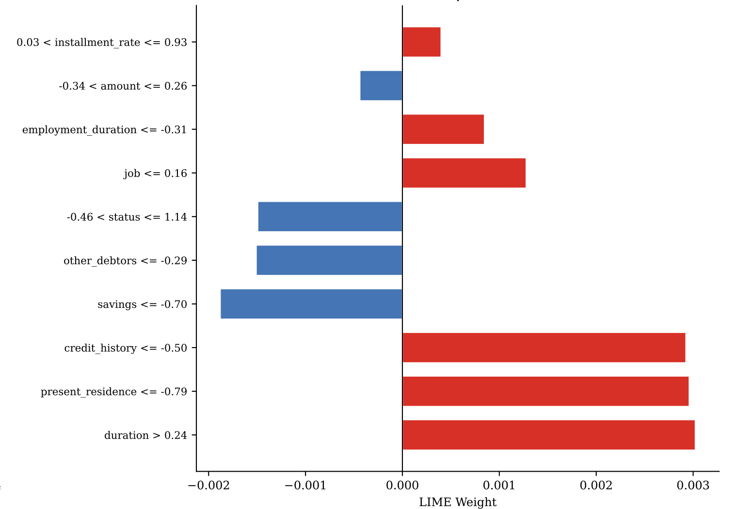
TN — idx 136 | P(def)=0.499
