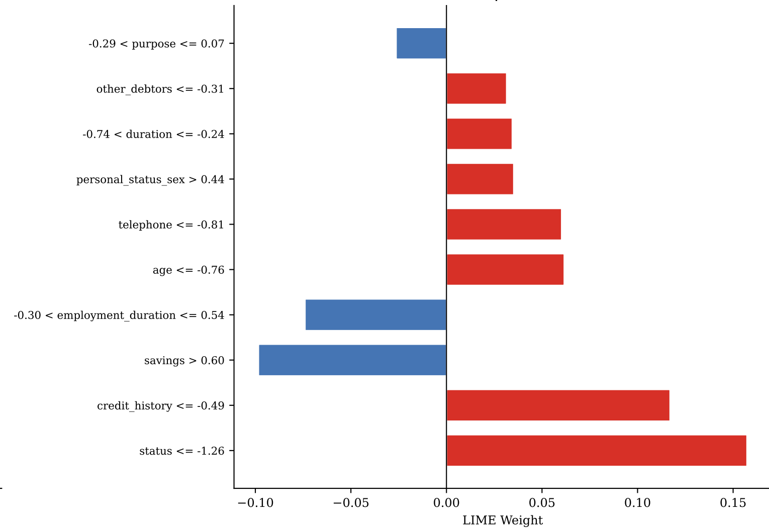
TN — idx 102 | P(def)=0.289
