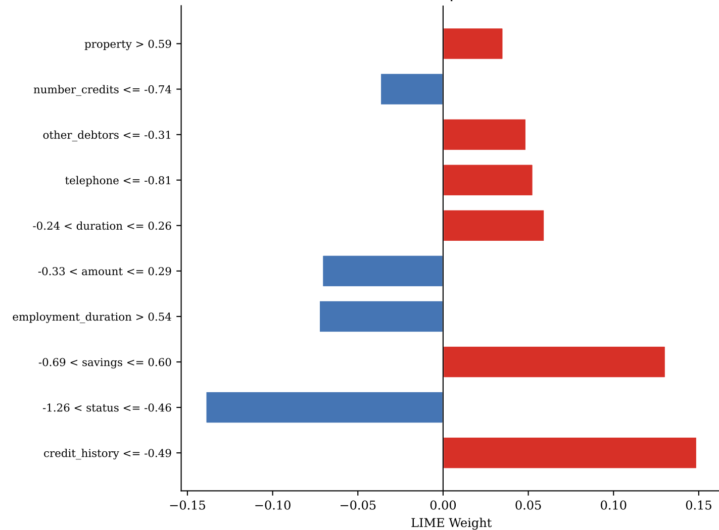
TN — idx 102 | P(def)=0.289
