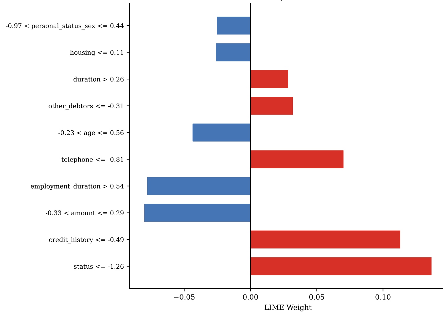
FN — idx 139 | P(def)=0.280
