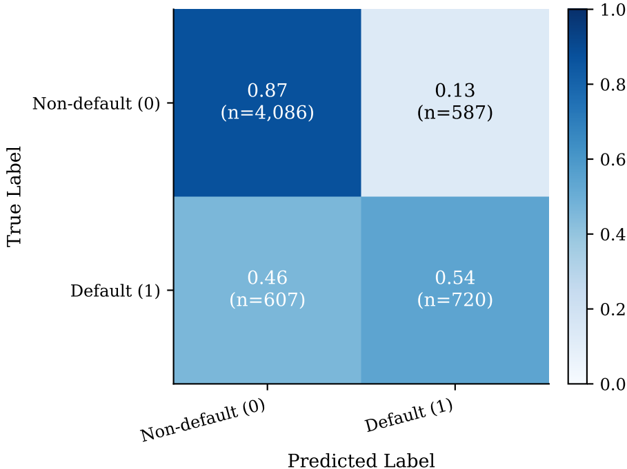
Confusion Matrix — XGBoost
