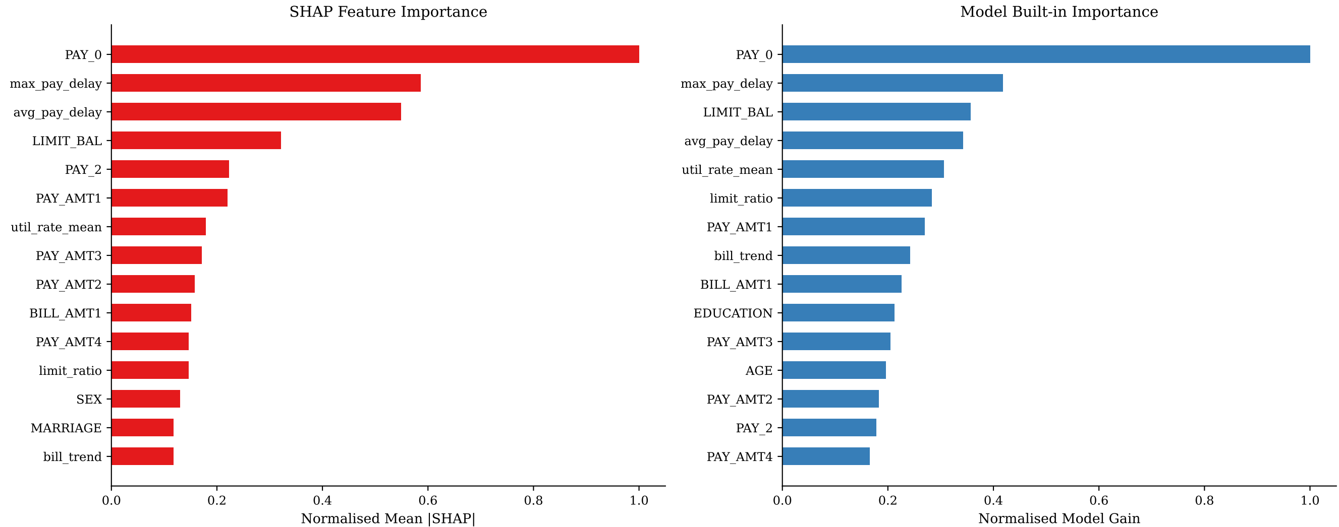
Feature Importance: SHAP vs. Model Gain (Top 15)
