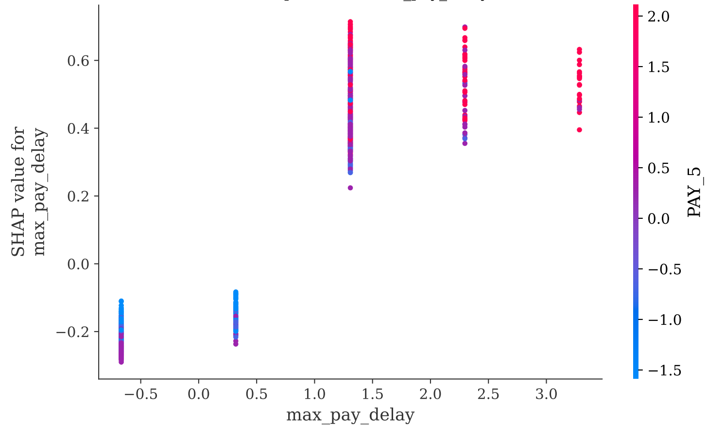
SHAP Dependence: max_pay_delay
