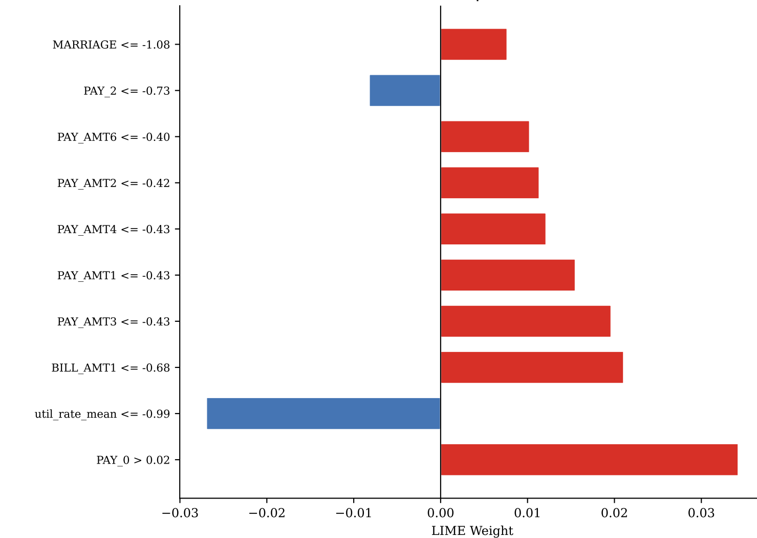
FN — idx 1423 | P(def)=0.299
