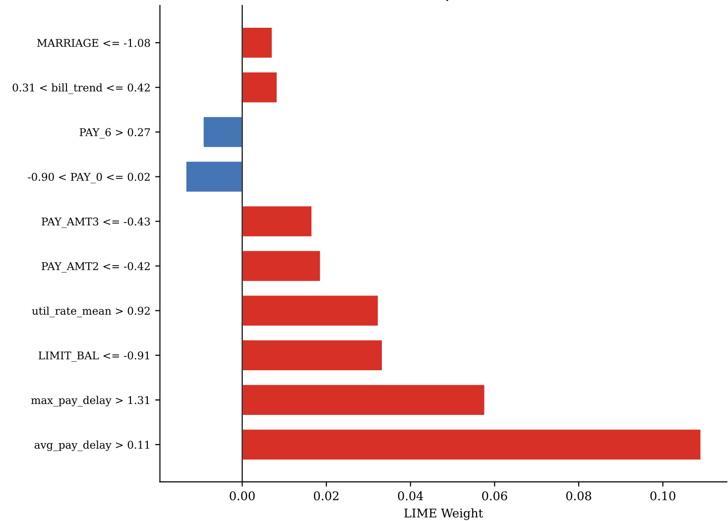
TN — idx 4892 | P(def)=0.300
