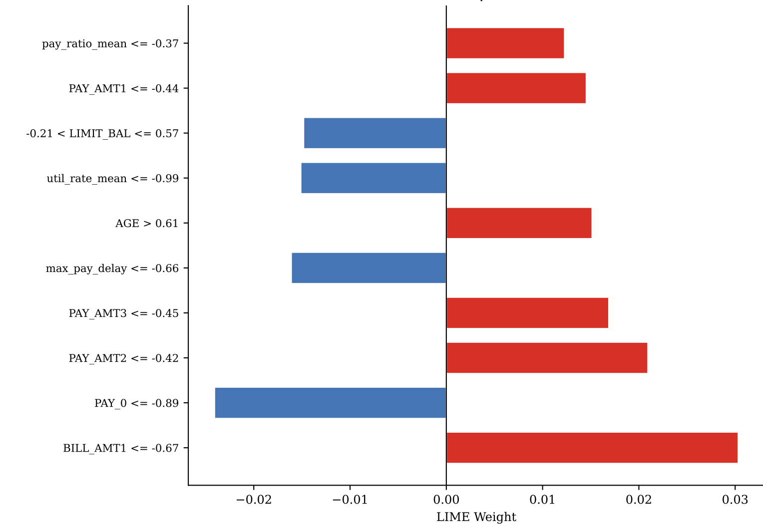
FN — idx 1557 | P(def)=0.270
