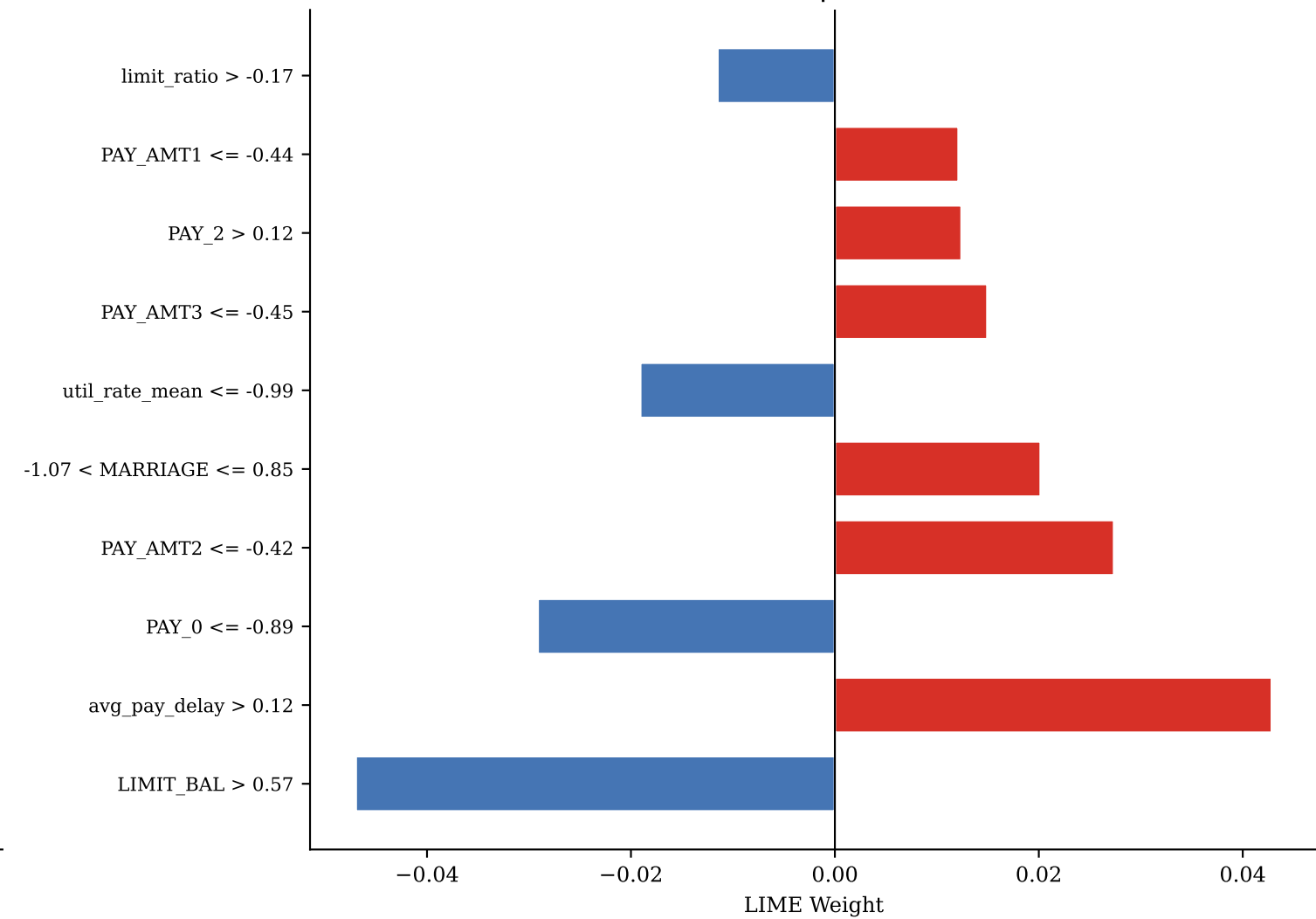
TN — idx 1314 | P(def)=0.270
