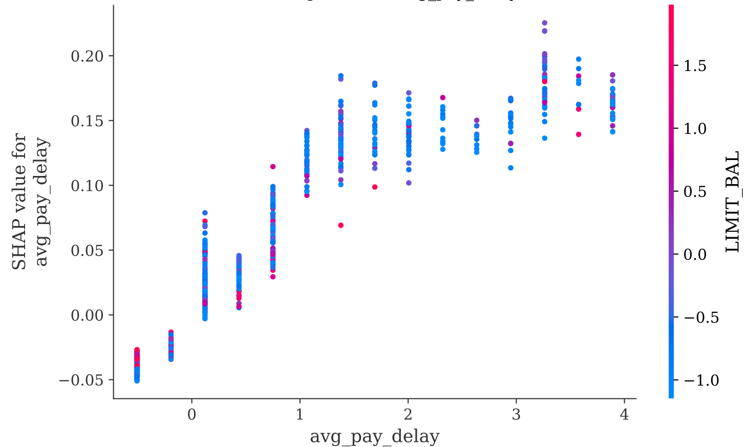
SHAP Dependence: avg_pay_delay
