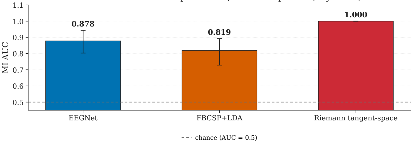
A5 black-box membership inference, victim comparison (PhysioNet)
