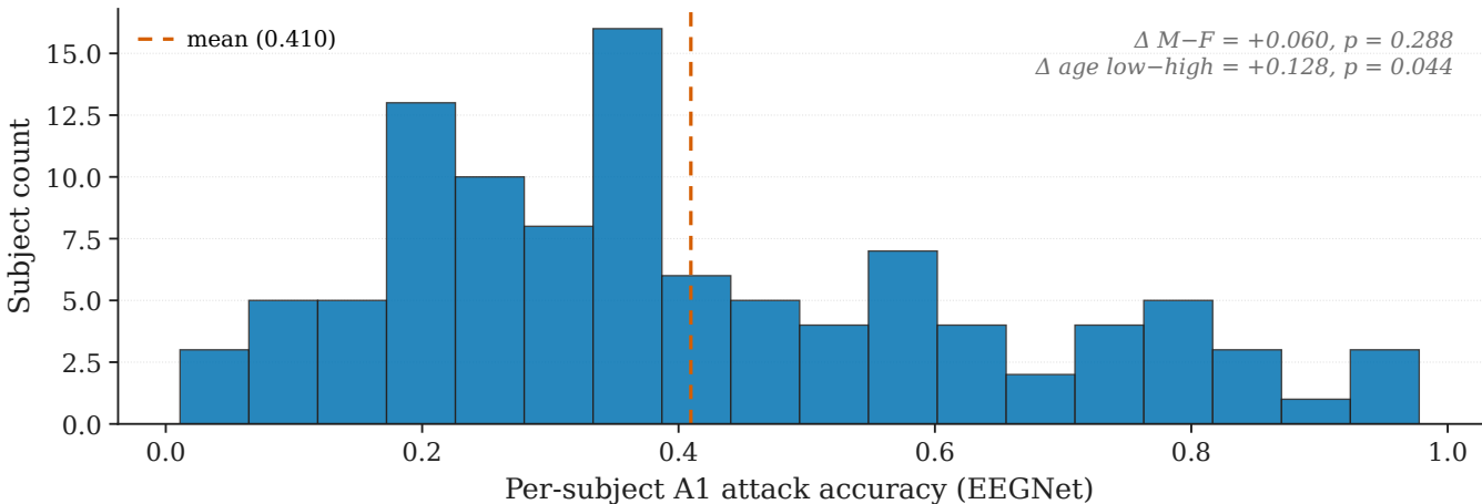
EEGNet within-cohort heterogeneity (PhysioNet, n=104)
