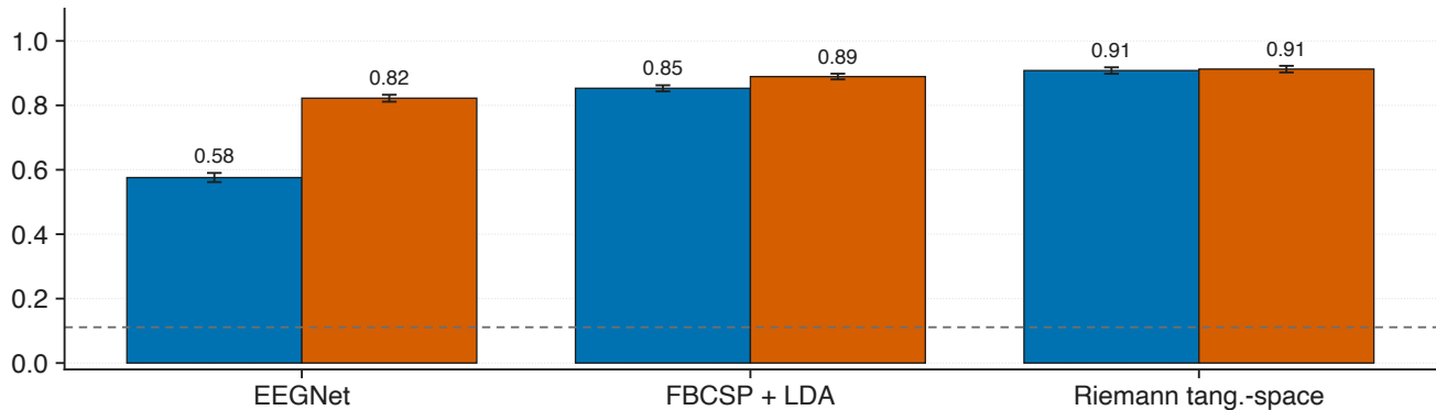
A3 cross-session re-ID (BCI IV-2a, n=9, session-1 session-2)
