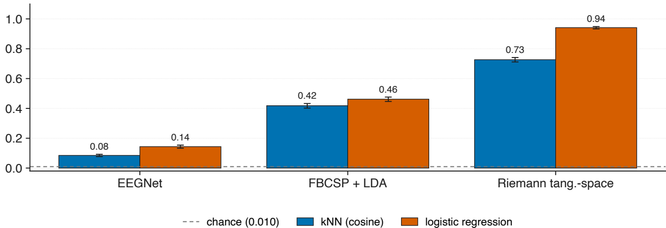
A2 cross-task re-ID with resting-state probe (PhysioNet, n=104)
