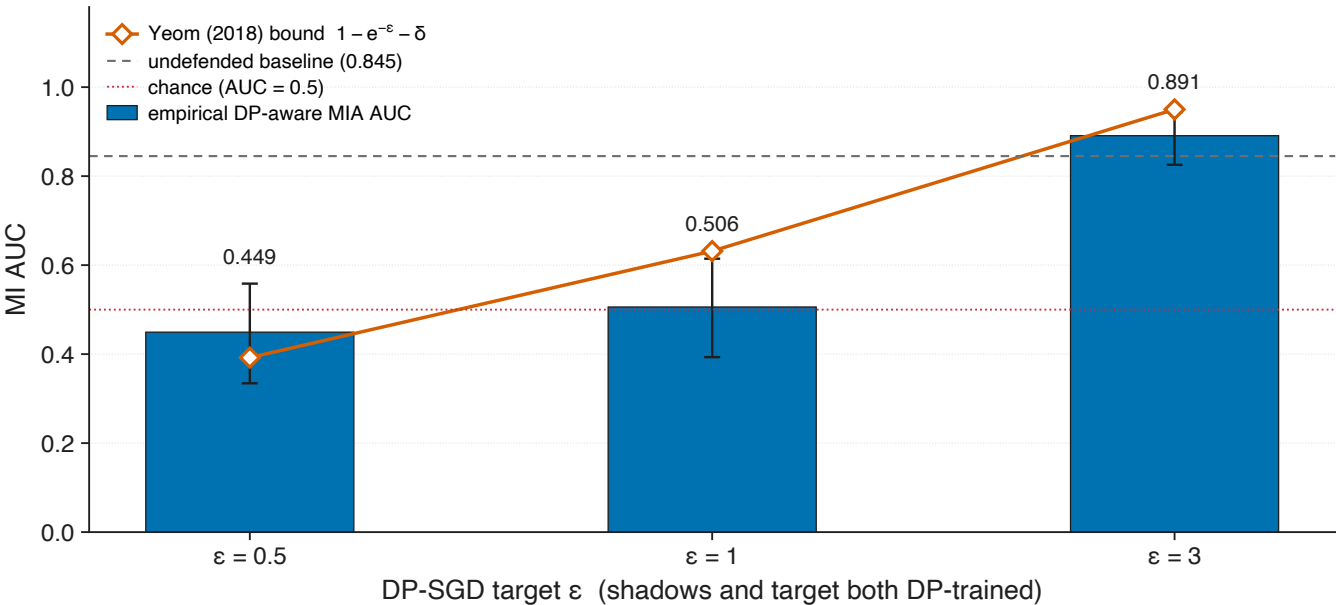
DP-aware membership inference vs Yeom (2018) bound across \epsilon (PhysioNet, EEGNet)
