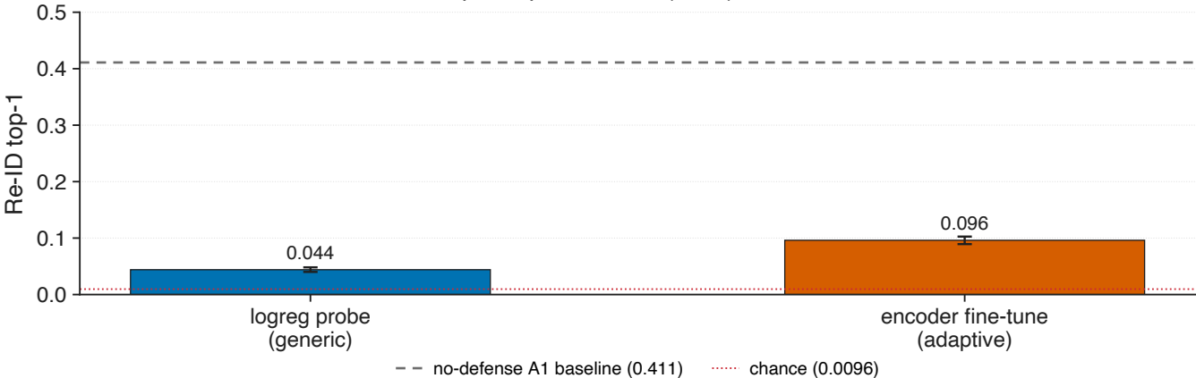
D4 federated DP-FedAvg (104 clients, 30 rounds, q=0.5 , \sigma=0.4 ) participant-level \epsilon (RDP) = 97.7
