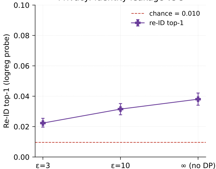
Privacy: identity leakage vs \epsilon
