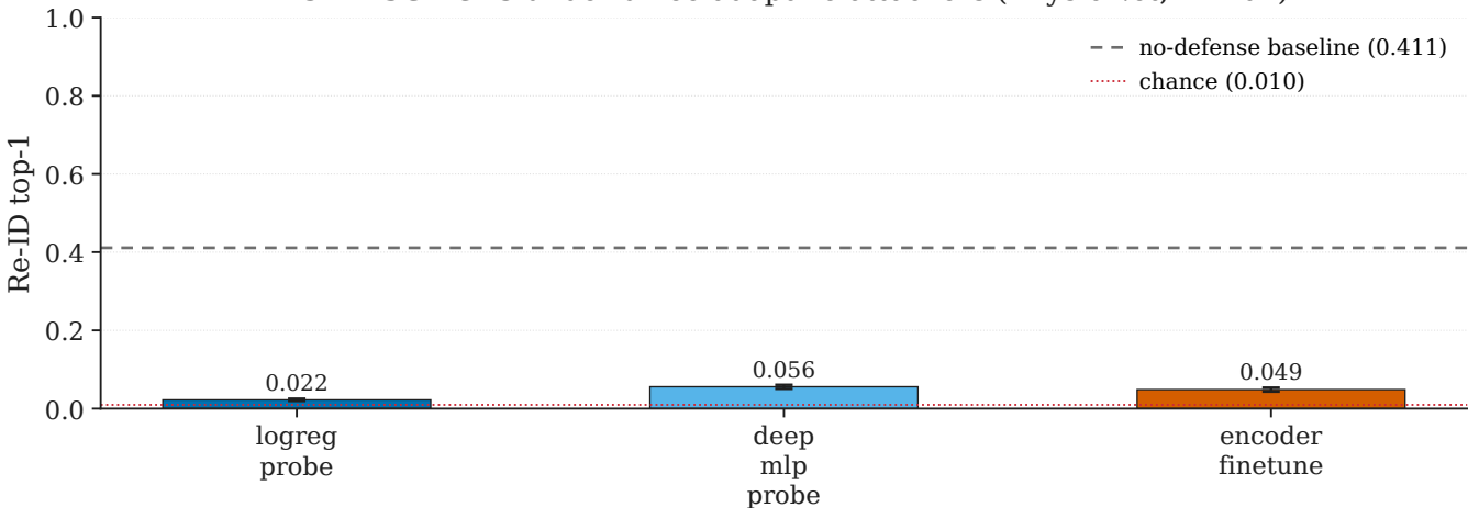
D3 DP-SGD \epsilon=3 under three adaptive attackers (PhysioNet, n=104)
