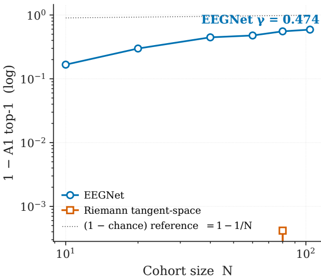
Re-ID scaling vs cohort size
