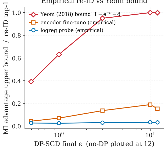
Empirical re-ID vs Yeom bound
