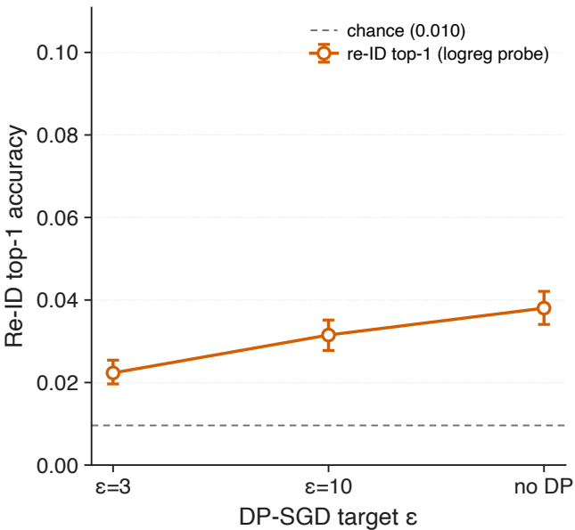
D3 DP-SGD \epsilon sweep, three-point grid
