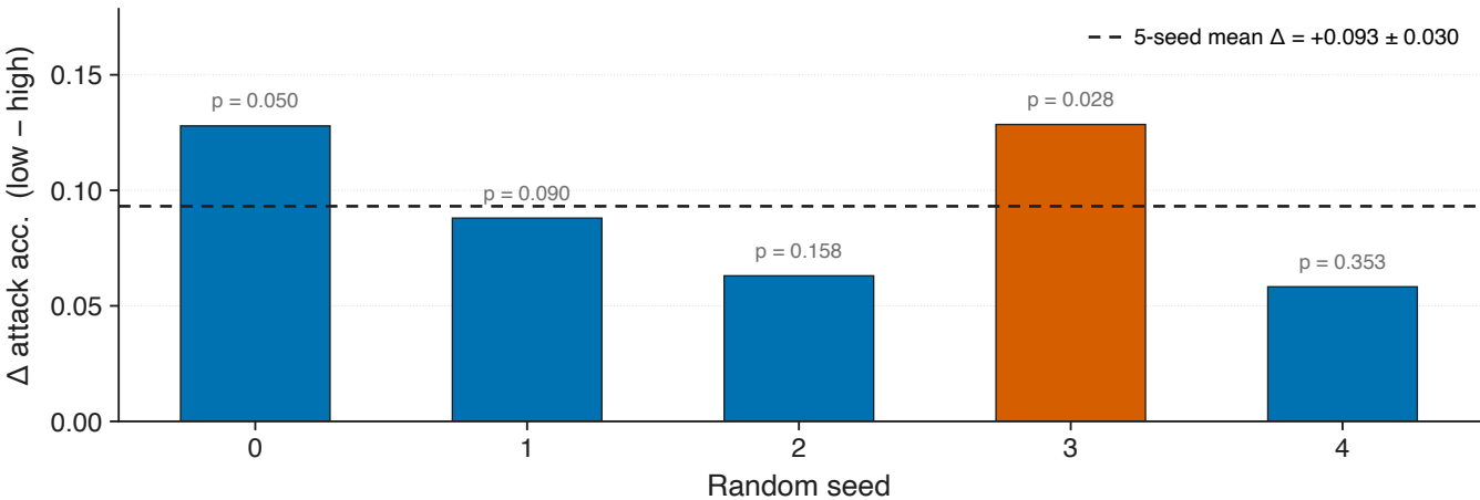
EEGNet age effect across 5 seeds (PhysioNet, n=91 age-known) · Fisher combined p = 0.0083
