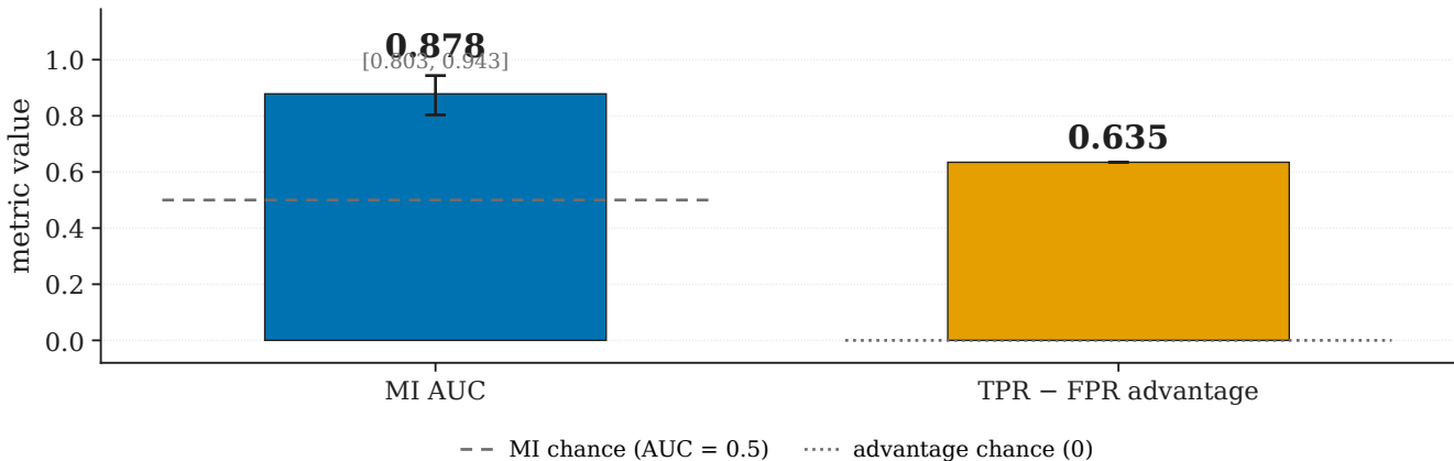
A5 black-box membership inference (PhysioNet, EEGNet shadows) 20 EEGNet shadows on PhysioNet imagery · 52 members vs 52 non-members
