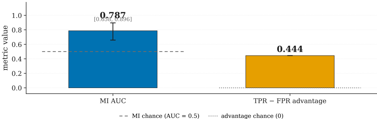
A5 black-box membership inference (Lee 2019) 12 EEGNet shadows on Lee 2019 imagery · 27 members vs 27 non-members
