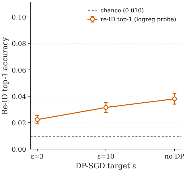
D3 DP-SGD \varepsilon sweep, milestone-era three-point grid
