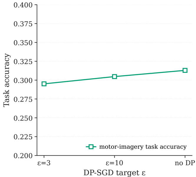
D3 DP-SGD \varepsilon sweep, milestone-era three-point grid
