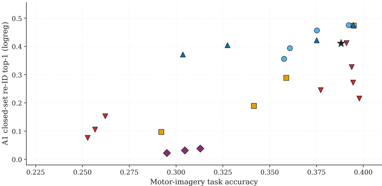
Privacy-utility Pareto across defense families (EEGNet victim)
