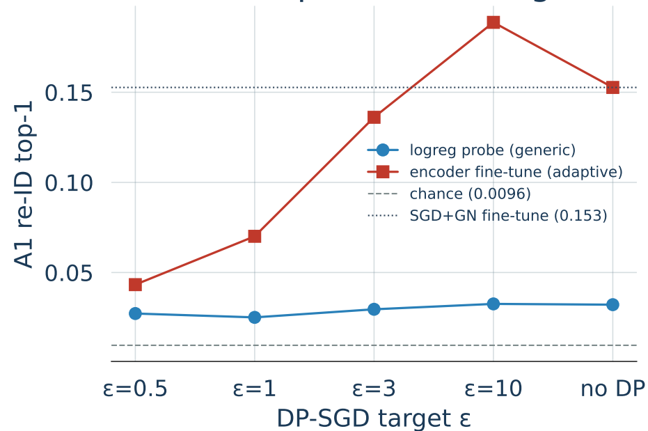
Re-ID top-1 vs DP budget
