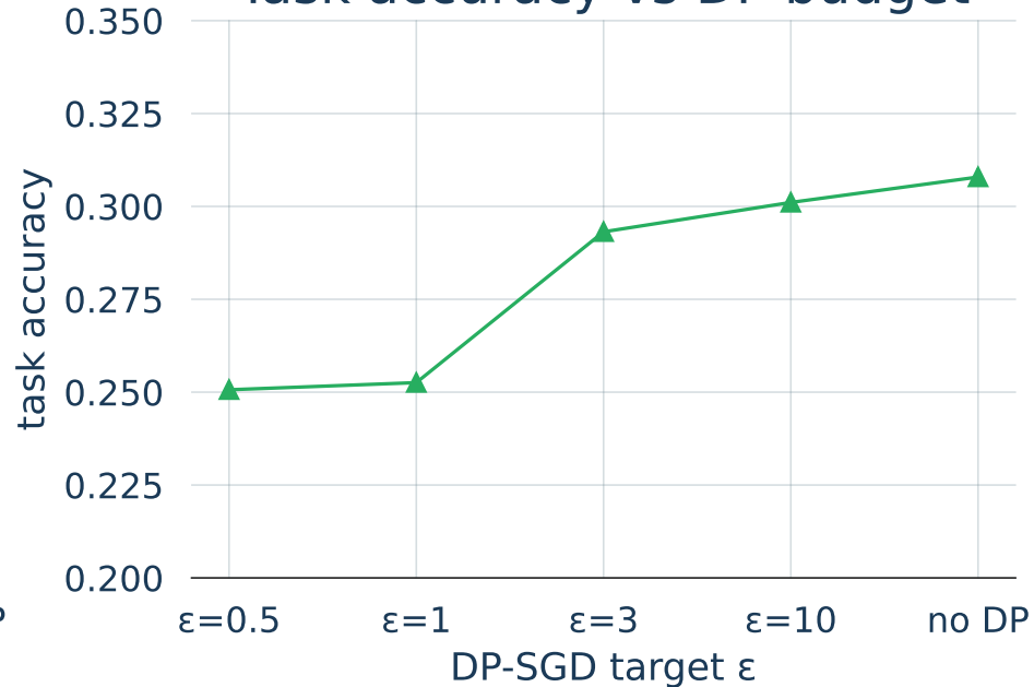
Task accuracy vs DP budget
