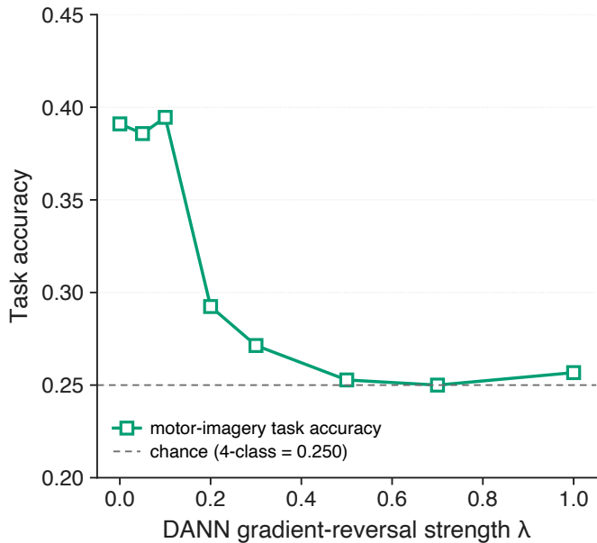
D2 DANN adversarial subject-invariance (EEGNet victim, n=104)
