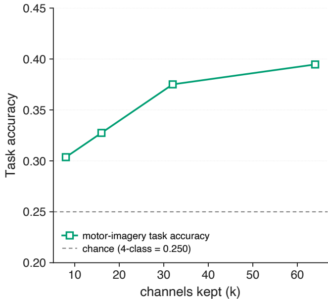
D1 channel-drop defense (top-k by variance, EEGNet victim, n=104)
