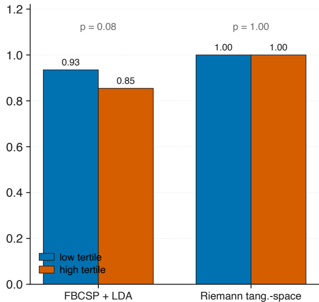
Age tertile stratification
