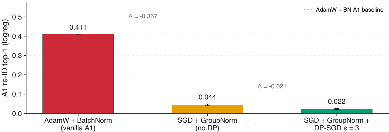
D3 architecture vs noise decomposition (EEGNet, PhysioNet n=104)
