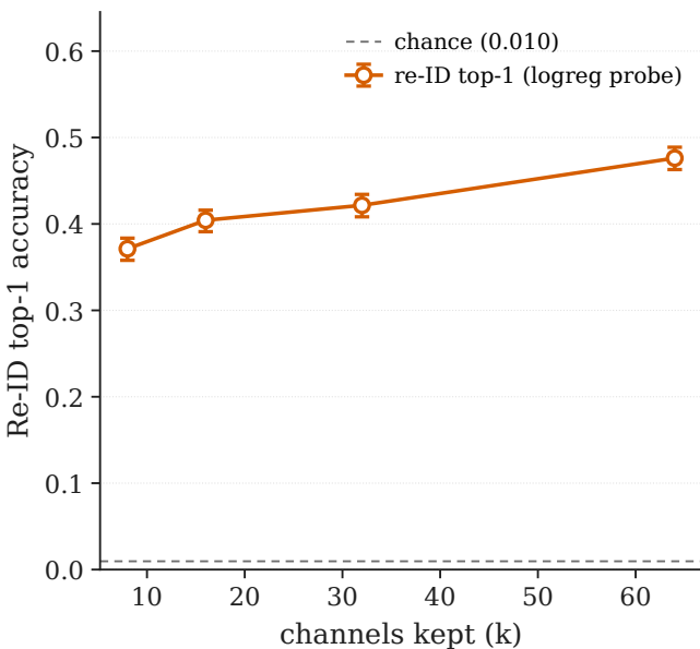
D1 channel-drop defense (top-k by variance, EEGNet victim, n=104)
