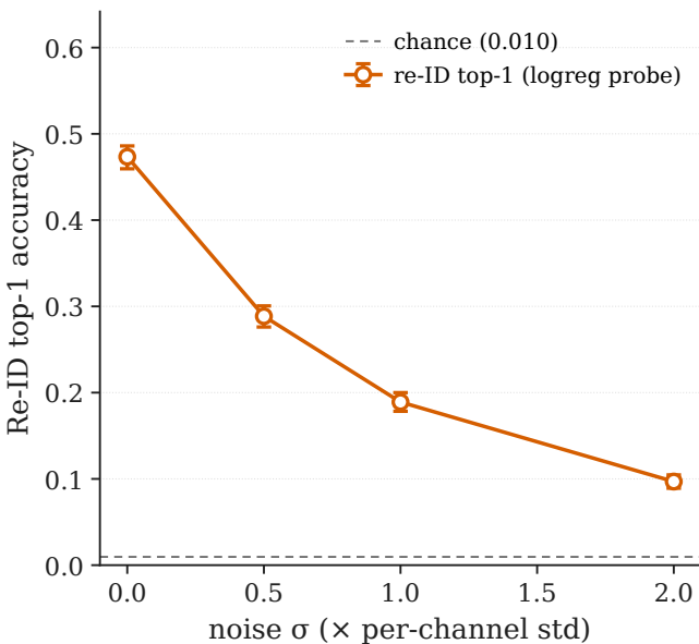
D1 additive Gaussian noise defense (EEGNet victim, n=104)
