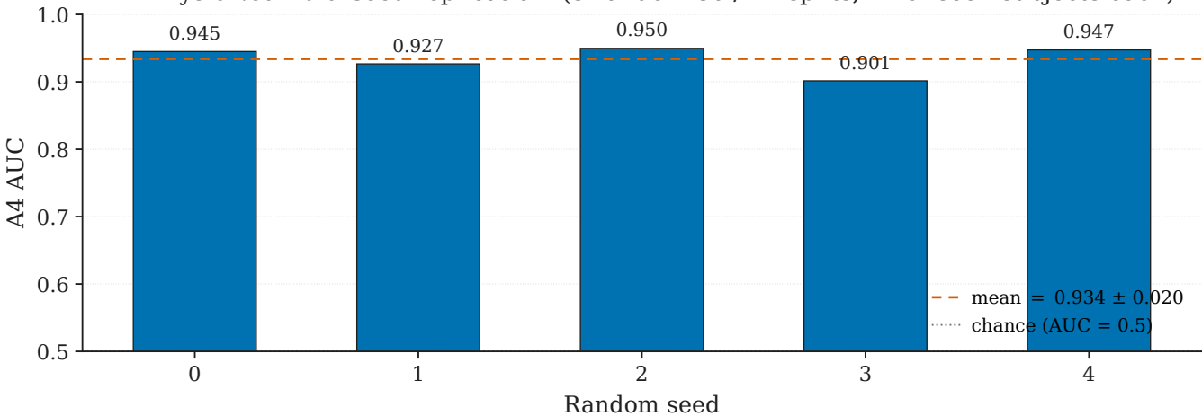
A4 PhysioNet multi-seed replication (5 random 80 / 24 splits, 24 unseen subjects each)
