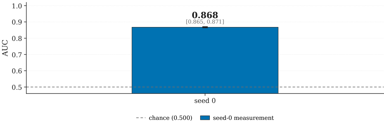
A4 open-set verification (Lee 2019, cross-session, 14 unseen subjects) trained on 40 subjects, 14 unseen, 50,000 pairs, EER = 0.216
