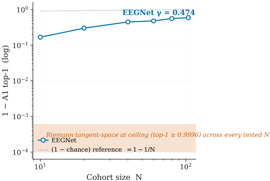
Re-ID scaling vs cohort size
