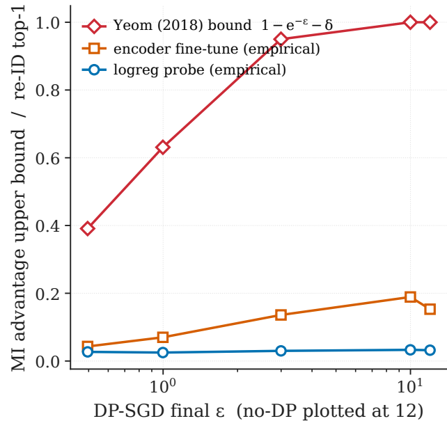
Empirical re-ID vs Yeom bound
