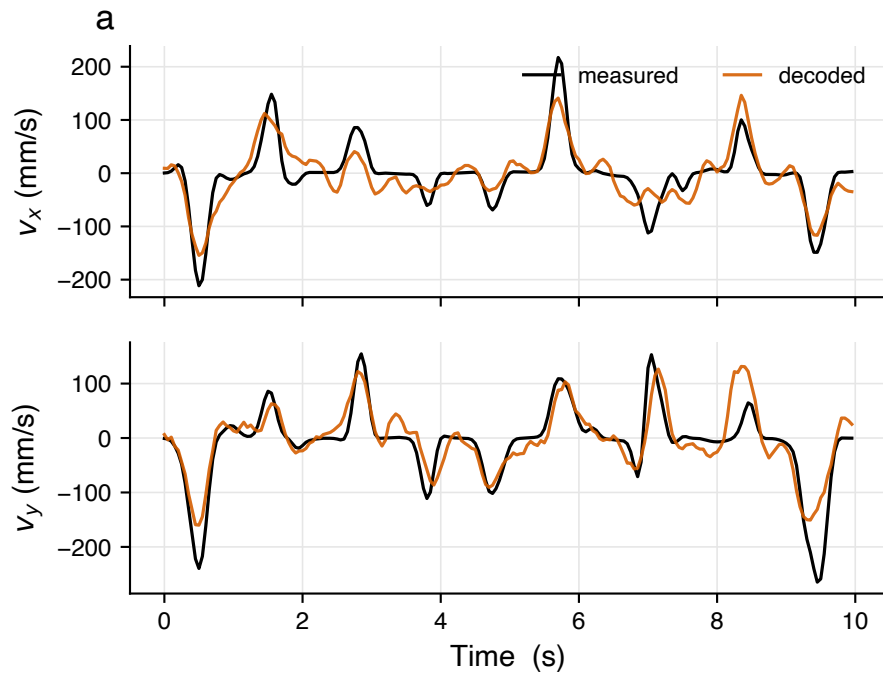
Trained SNN reconstruction ( f = 1 , R^2 = 0.68 )
