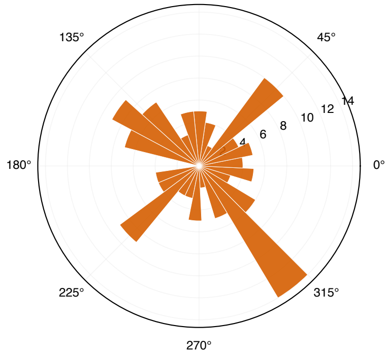
Trained-SNN hidden units ( H = 128 ) readout direction 90°
