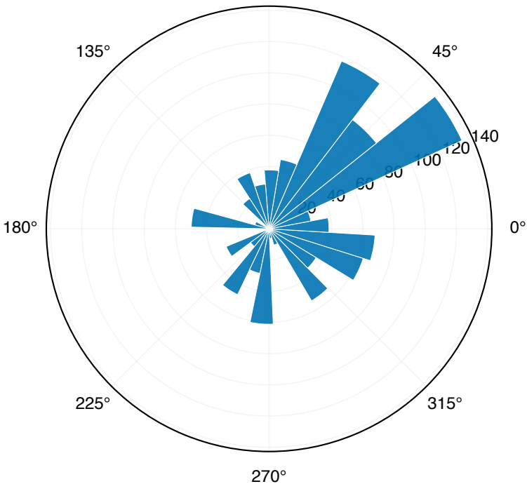
Input neurons ( N = 98 ) weighted by tuning depth 90°
