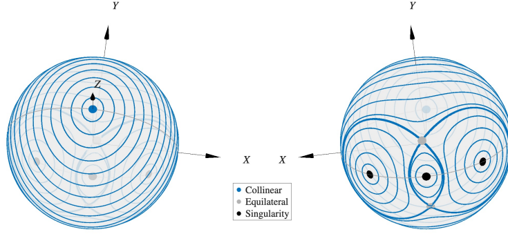
Figure 5.9: The phase portrait at point h with \Gamma_3 = 5 . Only the single collinear equilibrium \mathcal{E}_3 remains and is a center. The two equilateral triangular equilibria \mathcal{E}_{\text{tri}}^{\pm} are saddles.
