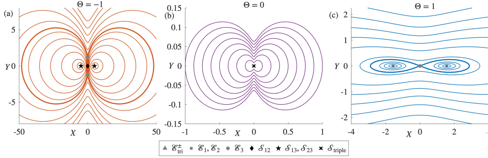
Figure 5.2: The XY phase planes of system at point b with \Gamma_3 = \frac{-3}{2} .
