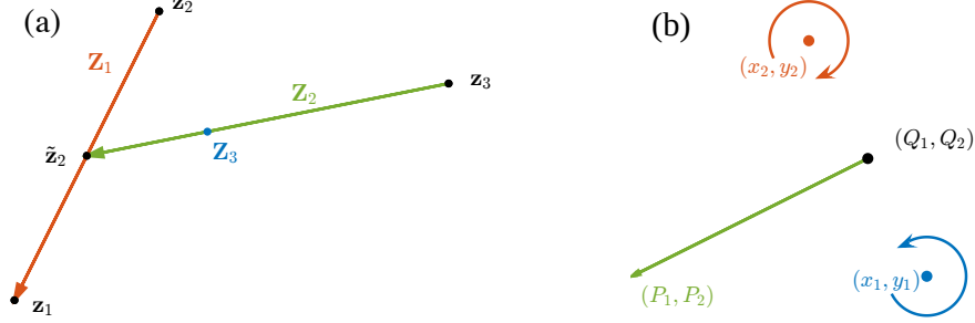
Figure 2.1: (a) Jacobi coordinates for three vortices with nonzero total circulation. The coordinate Z_1 is the vector from z_2 to z_1 , Z_2 is the vector from z_3 to the \tilde{z}_2 (the center of vorticity of the first two particles), and the transformed variable Z_3 is the conserved center of vorticity. (b) The alternative to Jacobi coordinates for two point-vortices with -\Gamma_2 = \Gamma_1 > 0 .
