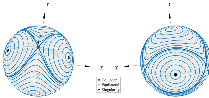
Figure 5.8: The phase portrait at point h with \Gamma_3 = \frac{1}{3} , showing “front” and “back” views of the sphere.
