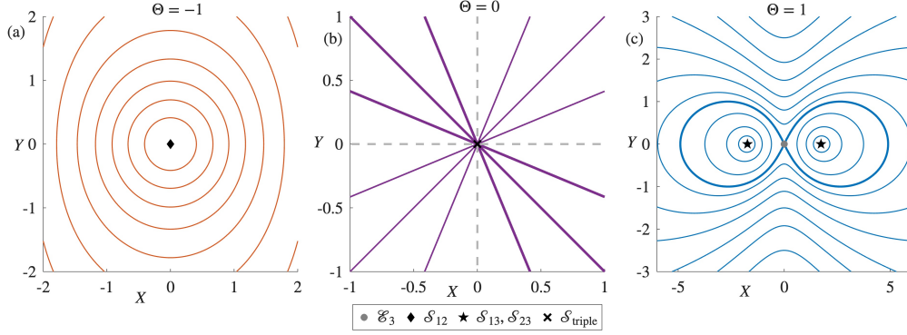
Figure 5.6: The XY phase planes at point e with \Gamma_3 = \frac{-1}{3} . The trajectories in the \Theta = 0 case are rays through the origin and correspond to triangles that shrink to zero in finite forward time (quadrants one and three), finite backward time (quadrants two and four), or do not change size (the X - and Y -axes).
