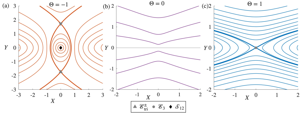
Figure 5.3: The XY phase planes at point c with \Gamma_3 = -1 . (a) The case \Theta < 0 with singularity \mathcal{S}_{12} at the origin and triangular configurations (X, Y, Z) at the intersections of the thick curves. (b) The case \Theta = 0 . The gray line Y = 0 is singular. (c) The case \Theta > 0 with collinear equilibrium at the origin.
