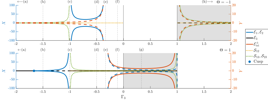
Figure 4.2: Bifurcation diagram displaying the equilibria and singularities defined by Eqs. (3.11), (4.3) and (4.10) for \Theta = -1 and \Theta = 1 as a function of \Gamma_3 along the vertical center line of Fig. 4.1. The X -component of the collinear equilibria and singularities is shown, using the y -axis scale on the left, and the Y component of the triangular equilibria is shown using the y -axis scale on the right. Dashed vertical lines show the \Gamma_1 values indicated by the letter labels in Fig. 4.1. Dashed equilibrium curves indicate instability. The points a and h lie outside the region plotted in this figure.
