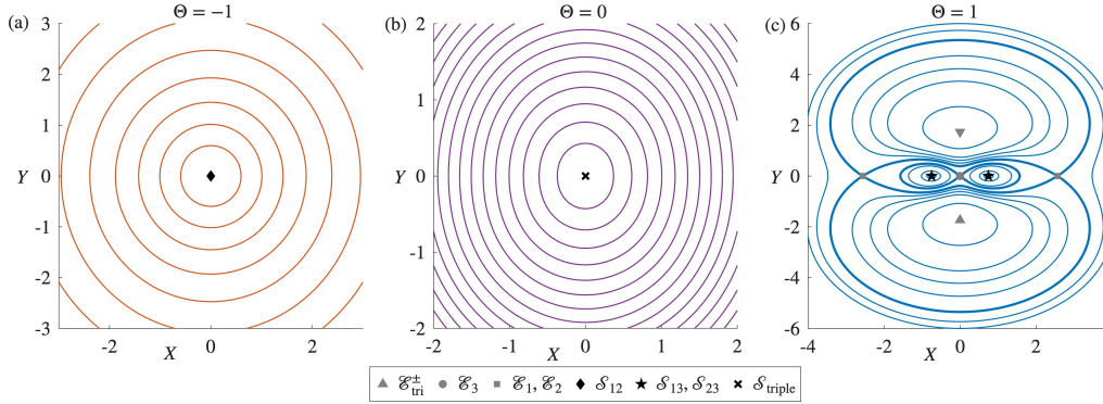
Figure 5.7: The XY phase planes in case f with \Gamma_3 = \frac{-1}{9} . (a) The case \Theta < 0 . (b) The case \Theta = 0 . (c) The case \Theta > 0 .
