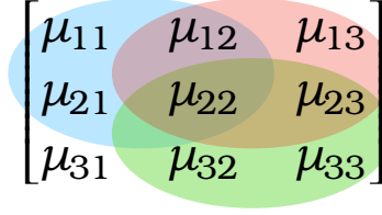
Figure 2.2: The three independent subdeterminants that must vanish in the case N = 3 .
