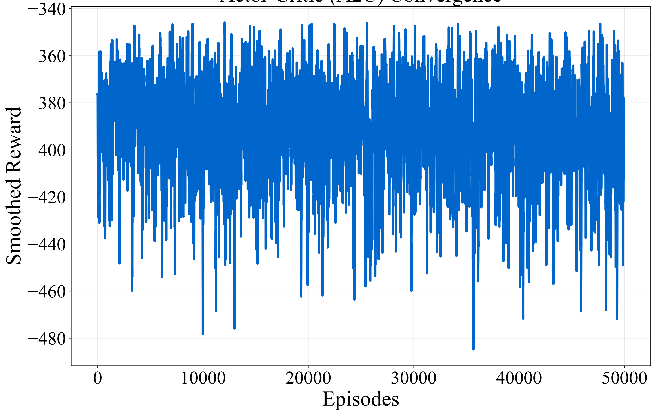
Actor-Critic (A2C) Convergence
