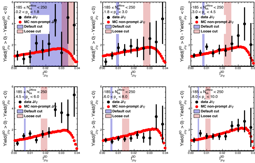
Figure 23: Comparison of the imbalance in \ell_{J/\psi}^{3D} distribution in pPb data for signal J/ψ from SPlot unfolding (black) and non-prompt J/ψ MC (red), for different p_T bins for 185 \leq N_{\text{trk}}^{\text{offline}} < 250 . All analysis cuts are applied except the \ell_{J/\psi}^{3D} cut. The \ell_{J/\psi}^{3D} cuts are indicated by color bands.
