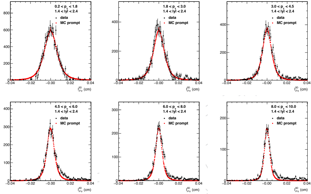
Figure 21: Comparison of the \ell_{J/\psi}^{3D} distribution in pPb data for signal J/\psi from SPlot unfolding (black) and prompt J/\psi MC (red), for different p_T bins for 185 \leq N_{\text{trk}}^{\text{offline}} < 250 . The MC distribution is normalized to the data in the range of -0.004 < \ell_{J/\psi}^{3D} < 0.004 cm. All analysis cuts are applied except the \ell_{J/\psi}^{3D} cut.
