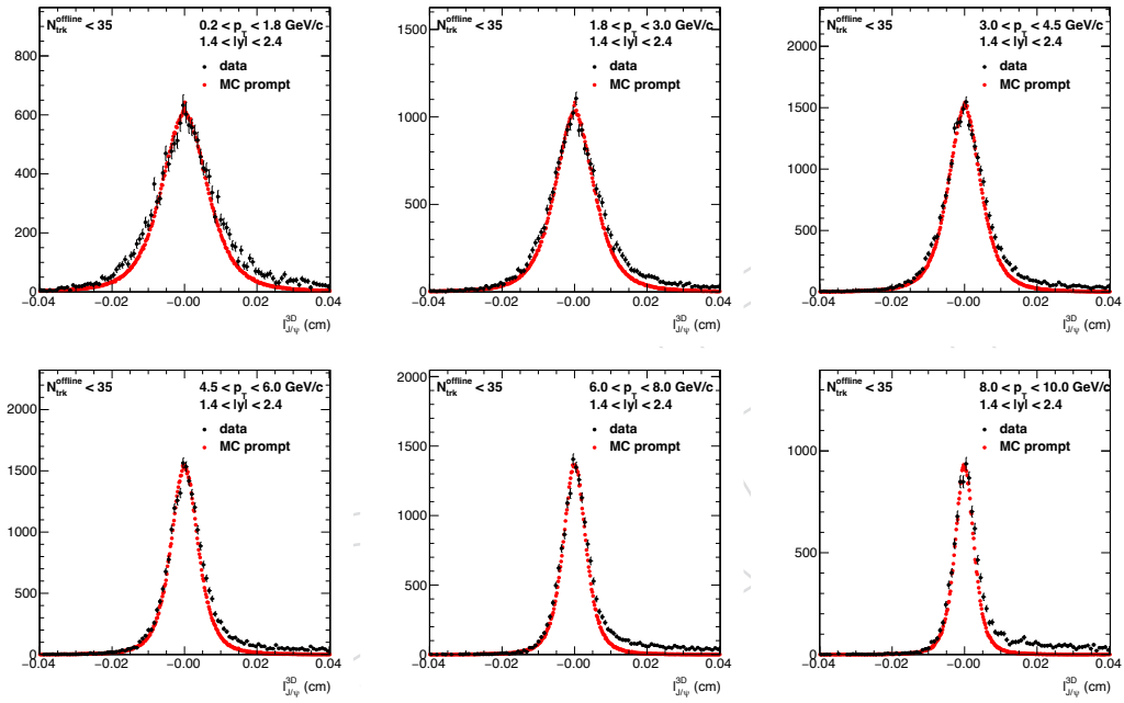
Figure 22: Comparison of the \ell_{J/\psi}^{3D} distribution in pPb data for signal J/\psi from SPlot unfolding (black) and prompt J/\psi MC (red), for different p_T bins for N_{\text{trk}}^{\text{offline}} < 35 . The MC distribution is normalized to the data in the range of -0.004 < \ell_{J/\psi}^{3D} < 0.004 cm. All analysis cuts are applied except the \ell_{J/\psi}^{3D} cut.
