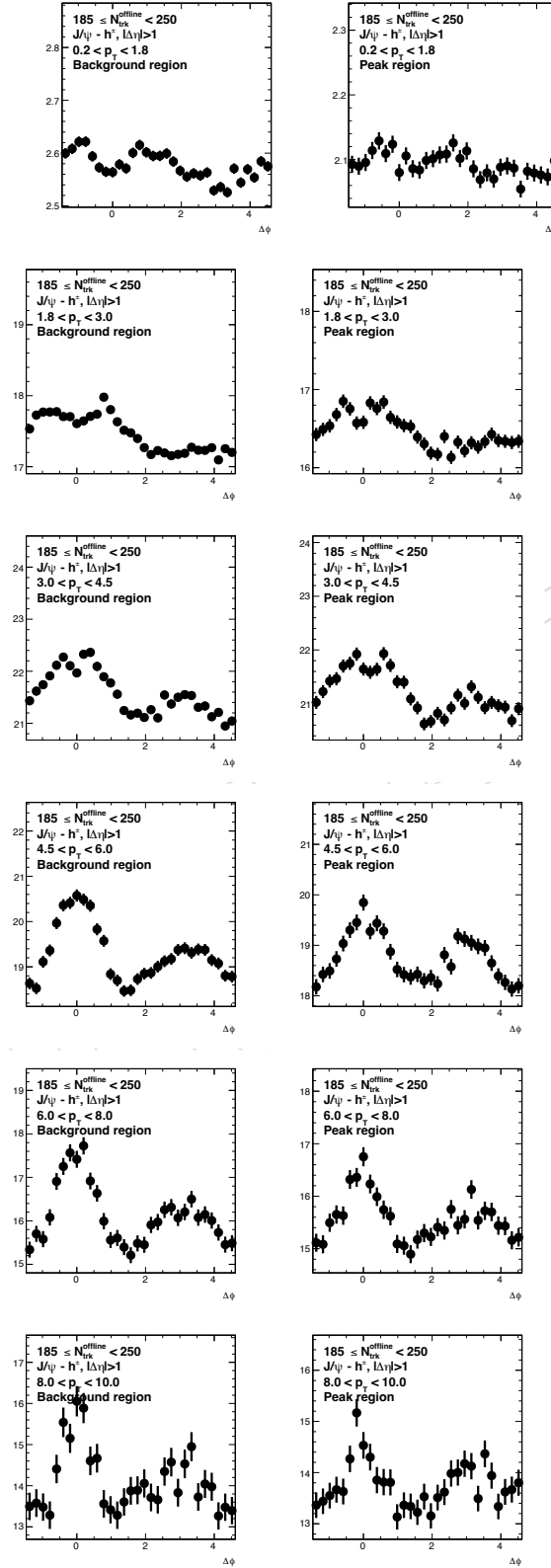
Figure 28: The near-side 1D projection of the J/\psi -hadron correlation functions for peak ( 2.94 < m_{\mu\mu} < 3.24 ) and background ( 2.55 < m_{\mu\mu} < 2.94 combined with 3.24 < m_{\mu\mu} < 3.63 ) mass regions for 185 \leq N_{\text{trk}}^{\text{offline}} < 250 .
