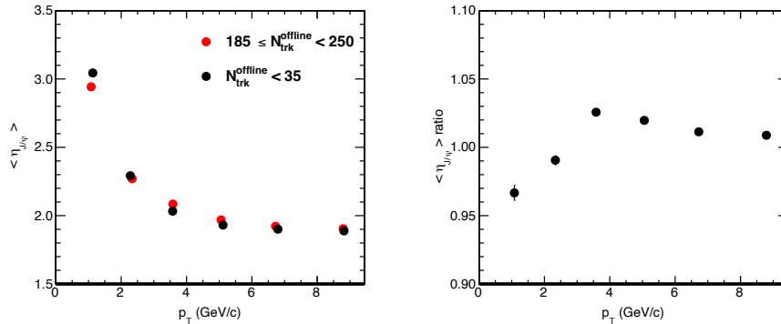
Figure 27: The average \eta of J/ψ candidates in each p_T bin for events with 185 \leq N_{\text{trk}}^{\text{offline}} < 250 and N_{\text{trk}}^{\text{offline}} < 35 (left), as well as their ratios (right).
