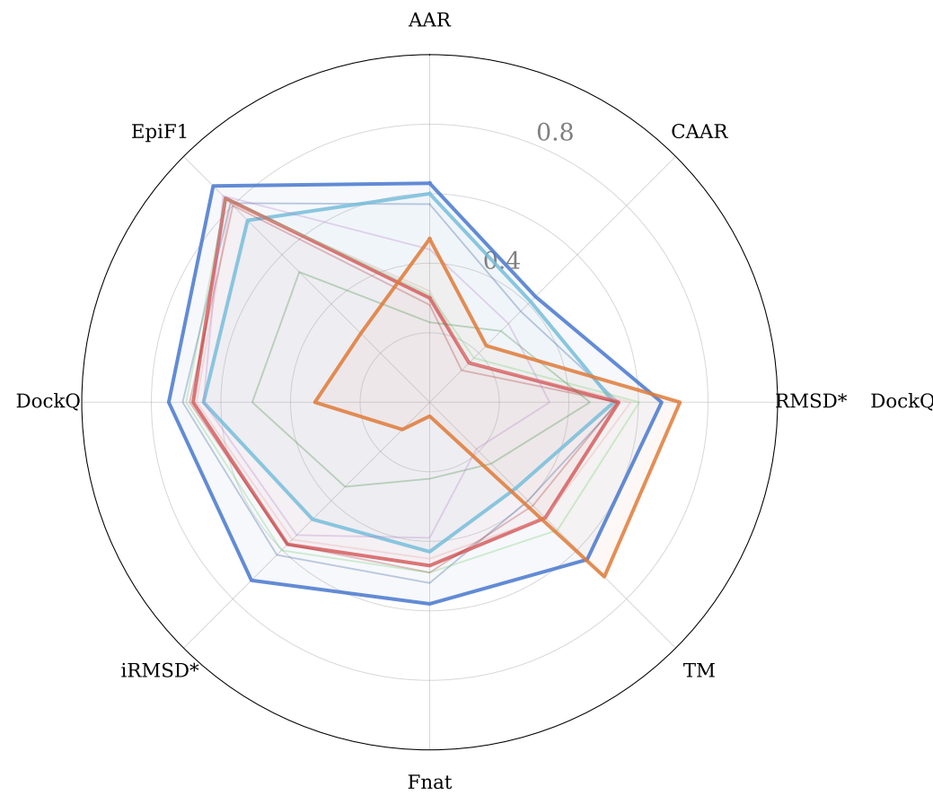
(b) CDR-H2
