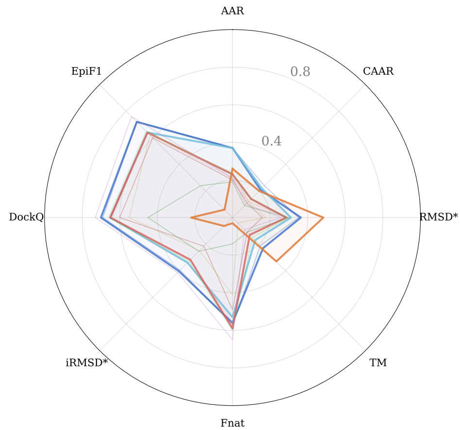
(c) CDR-H3
