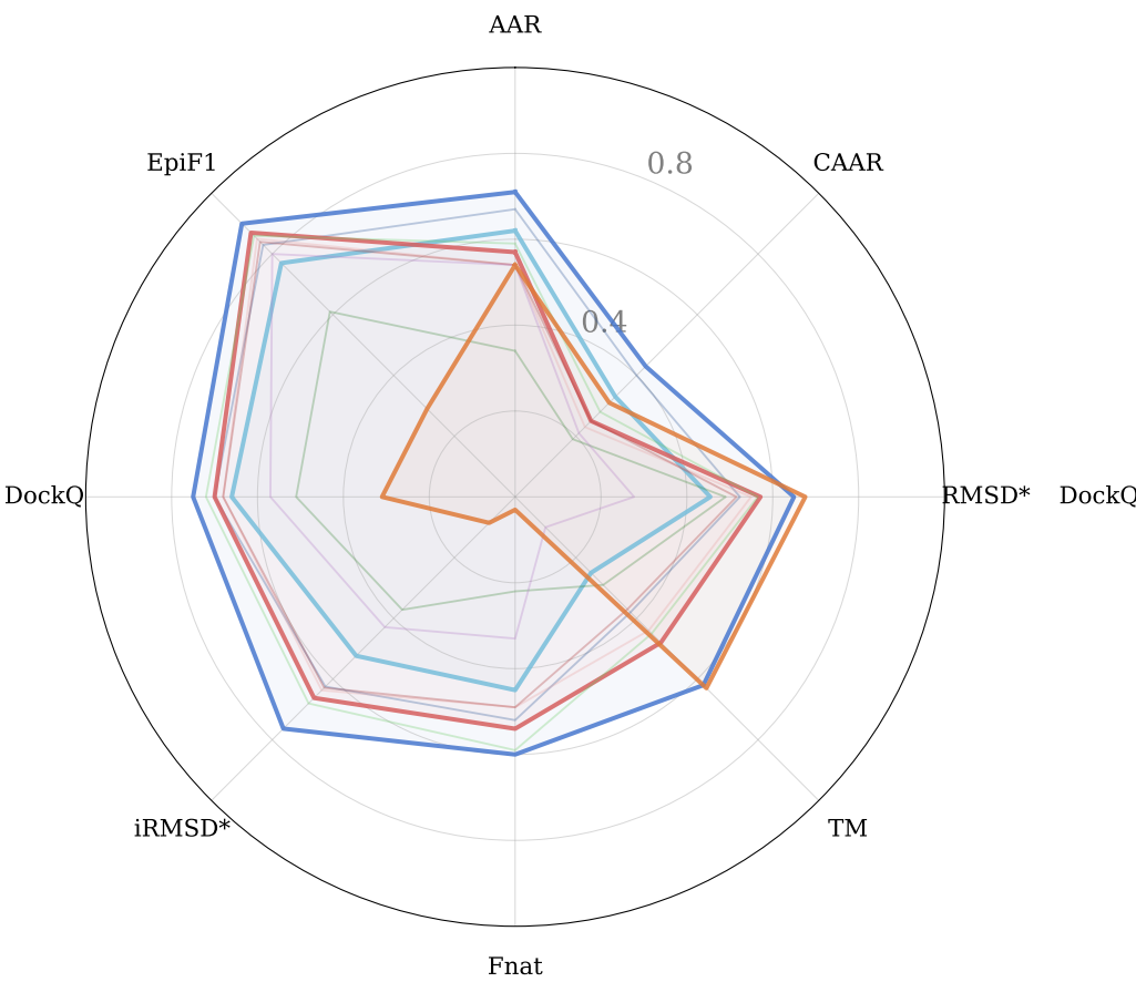
(a) CDR-H1
