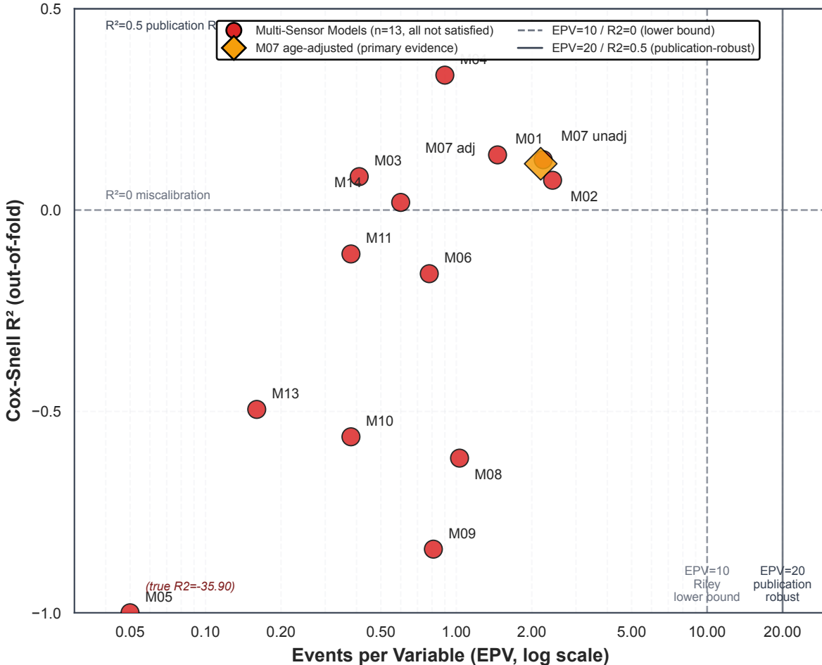
Figure 4: Riley 2020 Sample-Size Diagnostics (13 Multi-Sensor Models) All 13 not satisfying Riley standard; M07 age-adjusted highlighted
