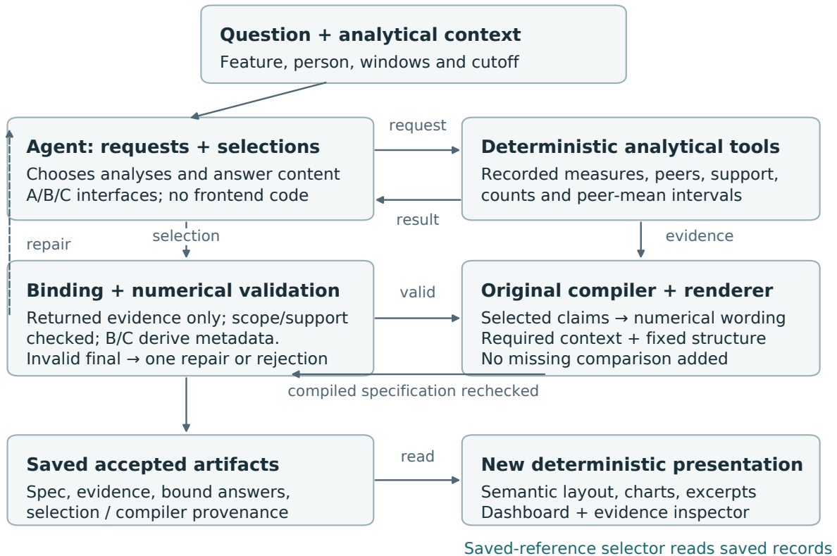
Figure 3: Implemented division of responsibilities, traced to the saved Stage 6 execution path. The model requests deterministic analyses and selects analytical answers; it does not author these layouts or unrestricted frontend code. Explicit binding in C resolves only returned evidence, while B and C derive redundant metadata. Numerical and scope checks can trigger a bounded repair or rejection. The original compiler supplies required structure and tagged context, but no missing comparison claim. The new presentation reads saved accepted artifacts and applies deterministic layouts and charts; its saved-reference selector does not call the model. Numerical validity and requested-answer completeness are separate properties. Completeness is assessed offline and remains subject to pending scientific review. This preparation stage executes none of the model or analytical investigation paths.
