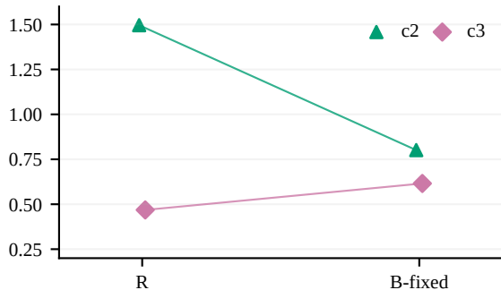
(b) S8, R / B-fixed: 2 pairs Higher-is-R AUC = 0.5
