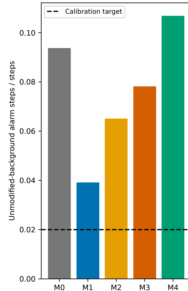
Realized negative-control alarms
