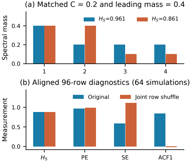
Fig. 2. Mathematical illustrations and aligned diagnostics, not primary fault performance. Equal average correlation and leading concentration can coexist with different spectral entropy. A joint time permutation preserves the evaluated matrix while temporal measurements can change.
