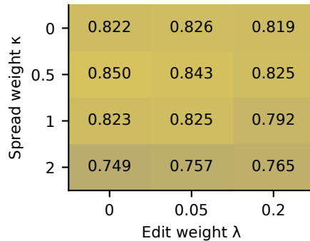
Synthetic 64 nonlinear
