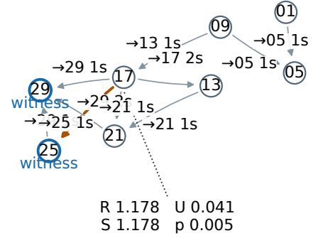
Fig. 2. An actual saved review case with fixed coordinates across the reference, observation-hypothesis and alternative-association panels. Saved S32N case from test_trajectory_3, sample interval [0, 64). Only a spike reading fault was injected. The strong alternative association mask illustrates diagnostic ambiguity. Graph version 7cc8c08c08e3b834. Arrows predict the labeled target at the stated lag in seconds. All highlighted sources and witnesses are retained. Context is a stored-relation spanning forest and layout uses no fault labels. This selected illustration does not estimate performance.
