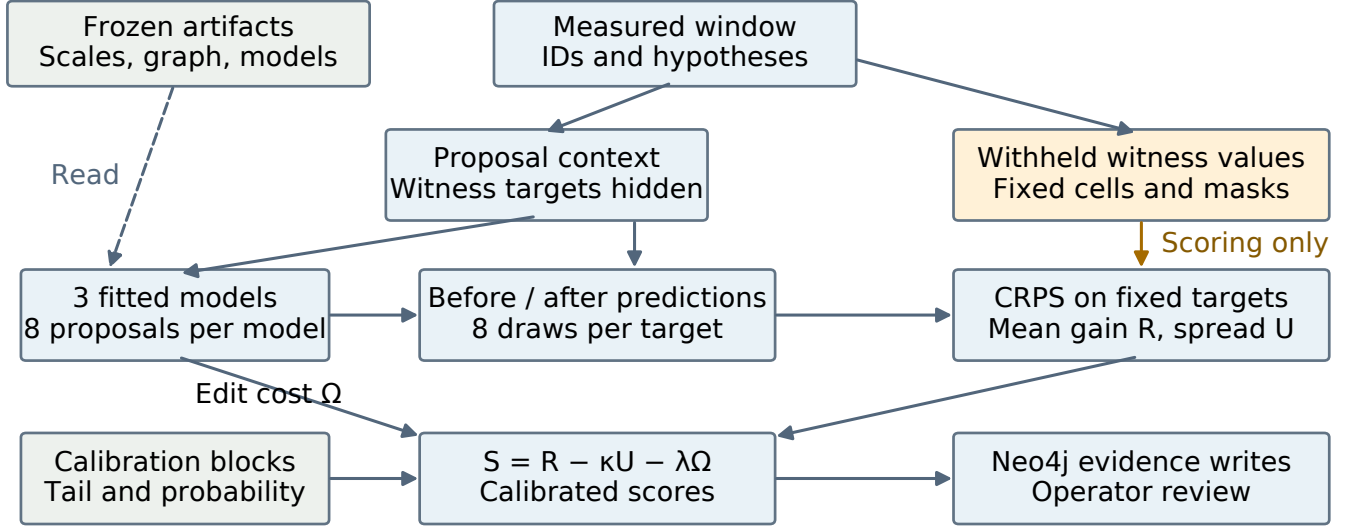
Fig. 1. Executed dataflow. Witness target values reach the loss calculation through a separate path. They do not enter repair generation. Training and calibration artifacts are frozen before test evaluation. Model reads and graph persistence have distinct roles.
