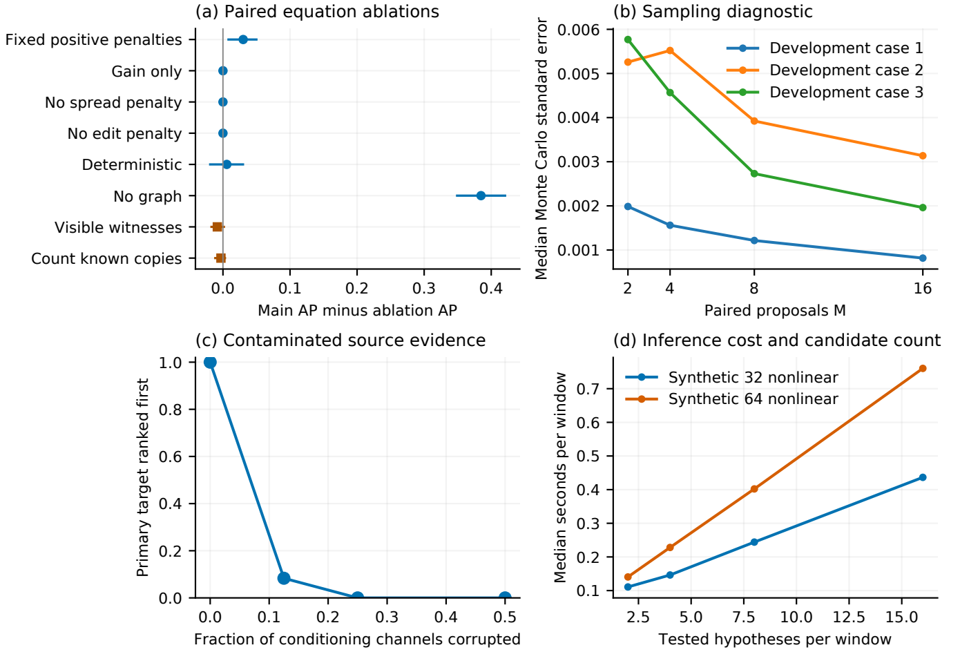
Fig. 4. Examination of the implemented score. Paired differences include block-bootstrap intervals. Sampling sensitivity uses development windows. Source contamination and computational tradeoffs come from separate saved runs. Unsafe evidence variants are identified explicitly.
